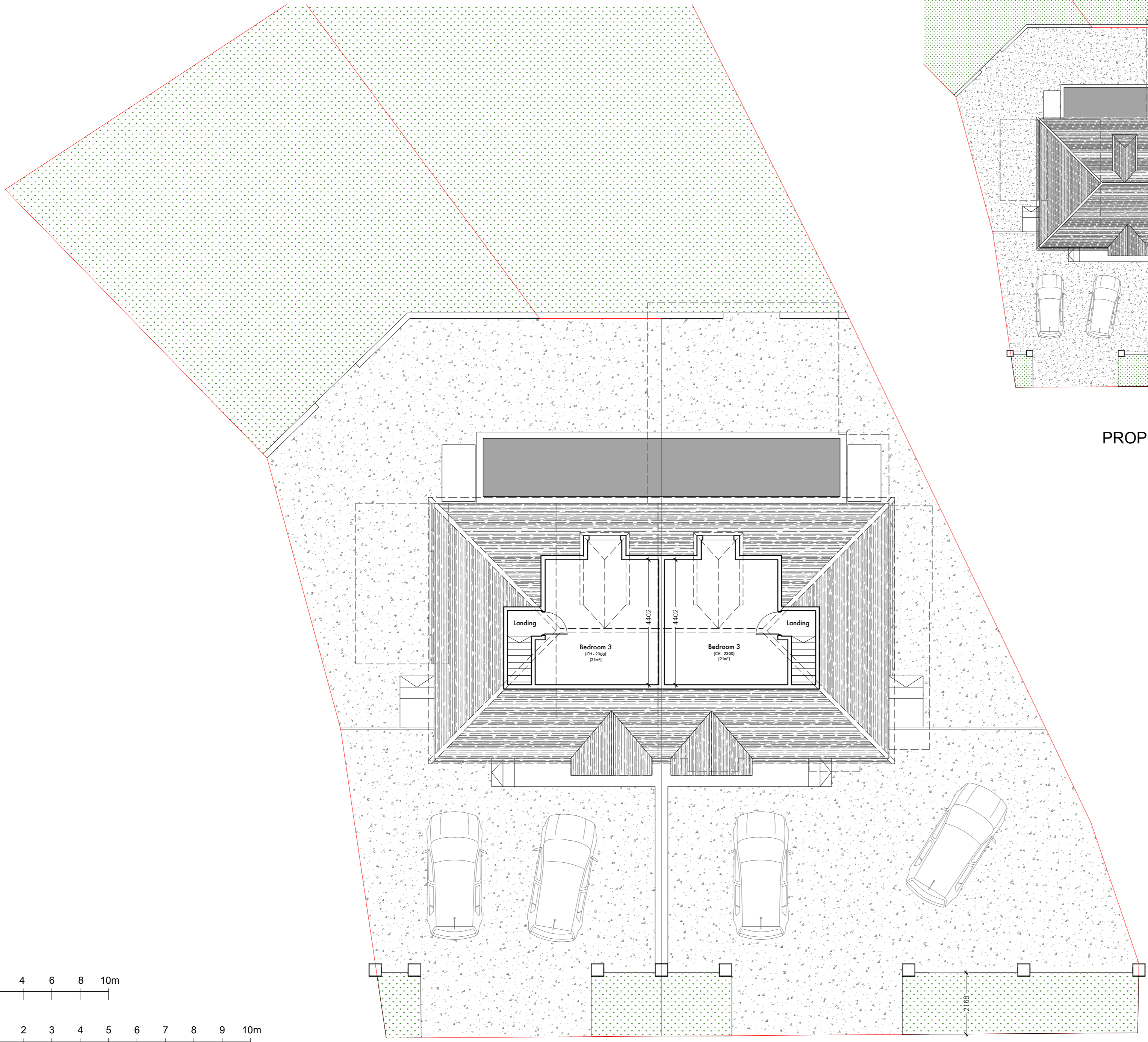
PROPOSED LOFT LEVEL
